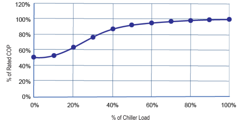
Existing Chiller Part Load Performance
