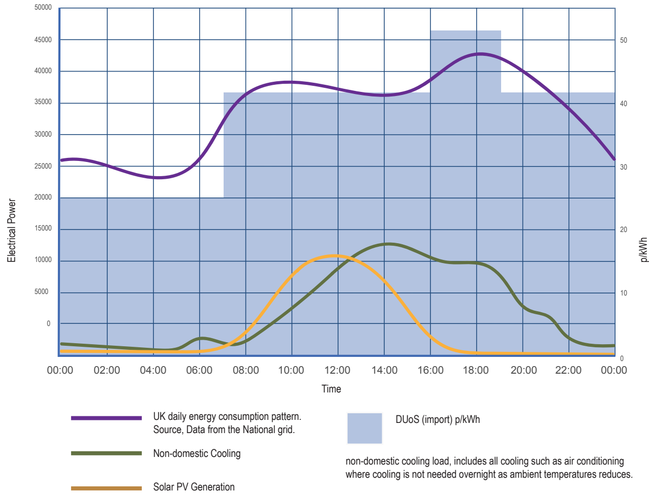
The relationship of energy consumption and production costs across a typical day in the UK Source: Cooling in the UK, BEIS 2021
